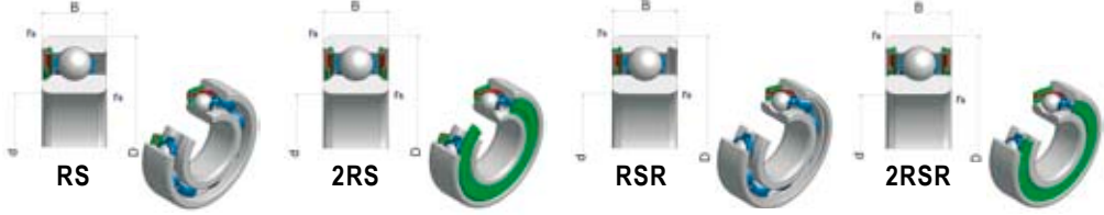
SINGLE ROW DEEP GROOVE BALL BEARINGS/SINGLE ROW DEEP GROOVE BALL BEARINGS WITH SHIELD AND SEAL/SINGLE ROW DEEP GROOVE BALL BEARINGS WITH SNAP RING GROOVE
