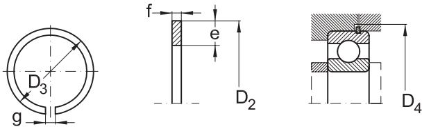
Snap ring
