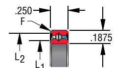
⑤ F = .015 Bearing corners are normally chamfered
