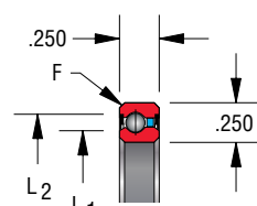
⑤ F = .025 Bearing corners are normally chamfered
