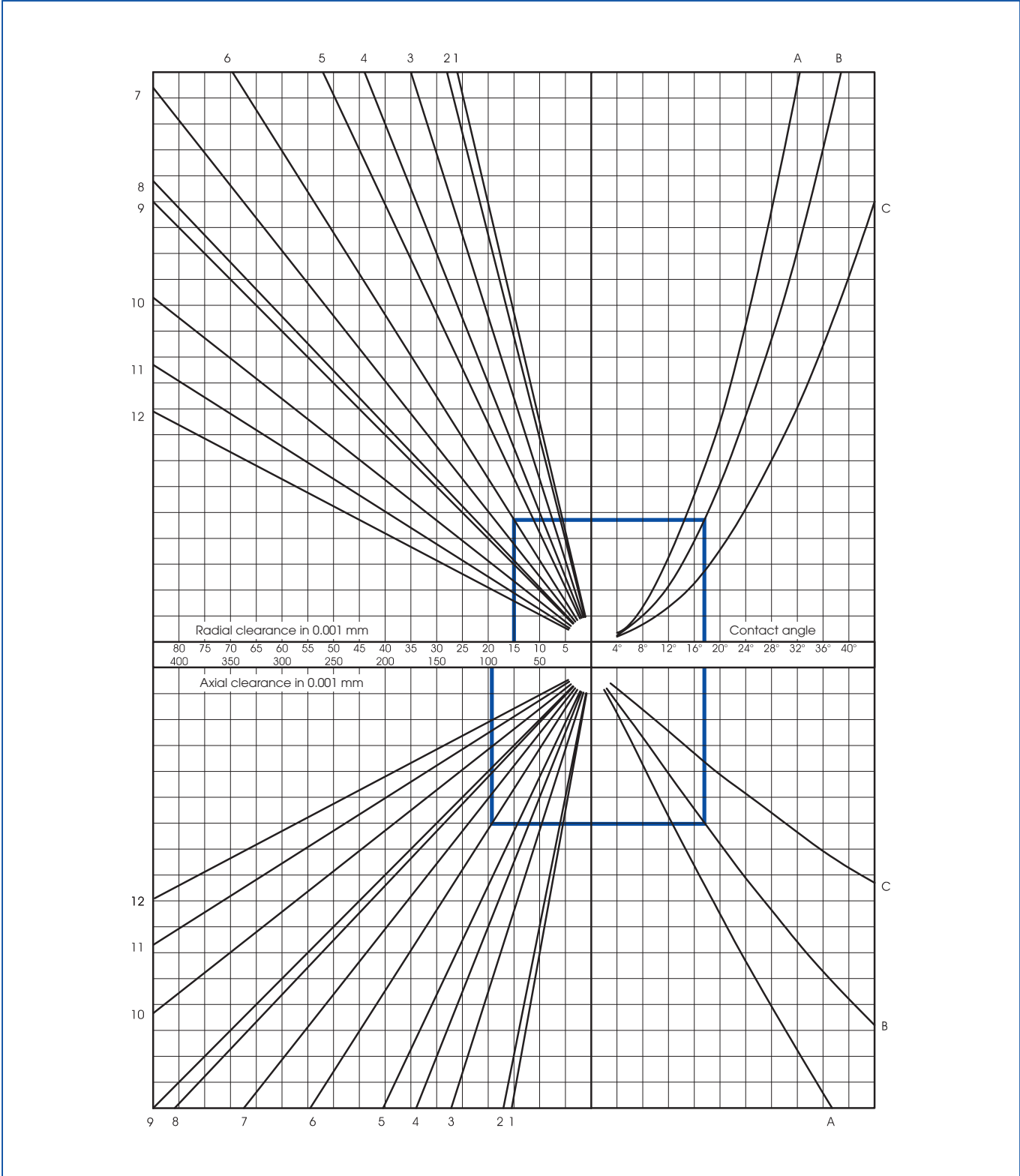
Figure 20: Contact angle and axial clearance
