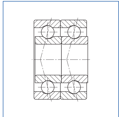
Figure 23: Tandem
