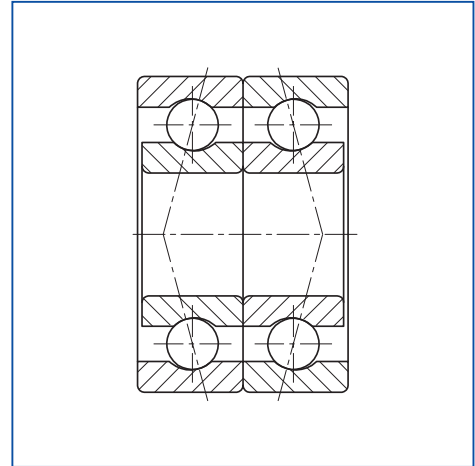
Figure 21: Back to back
