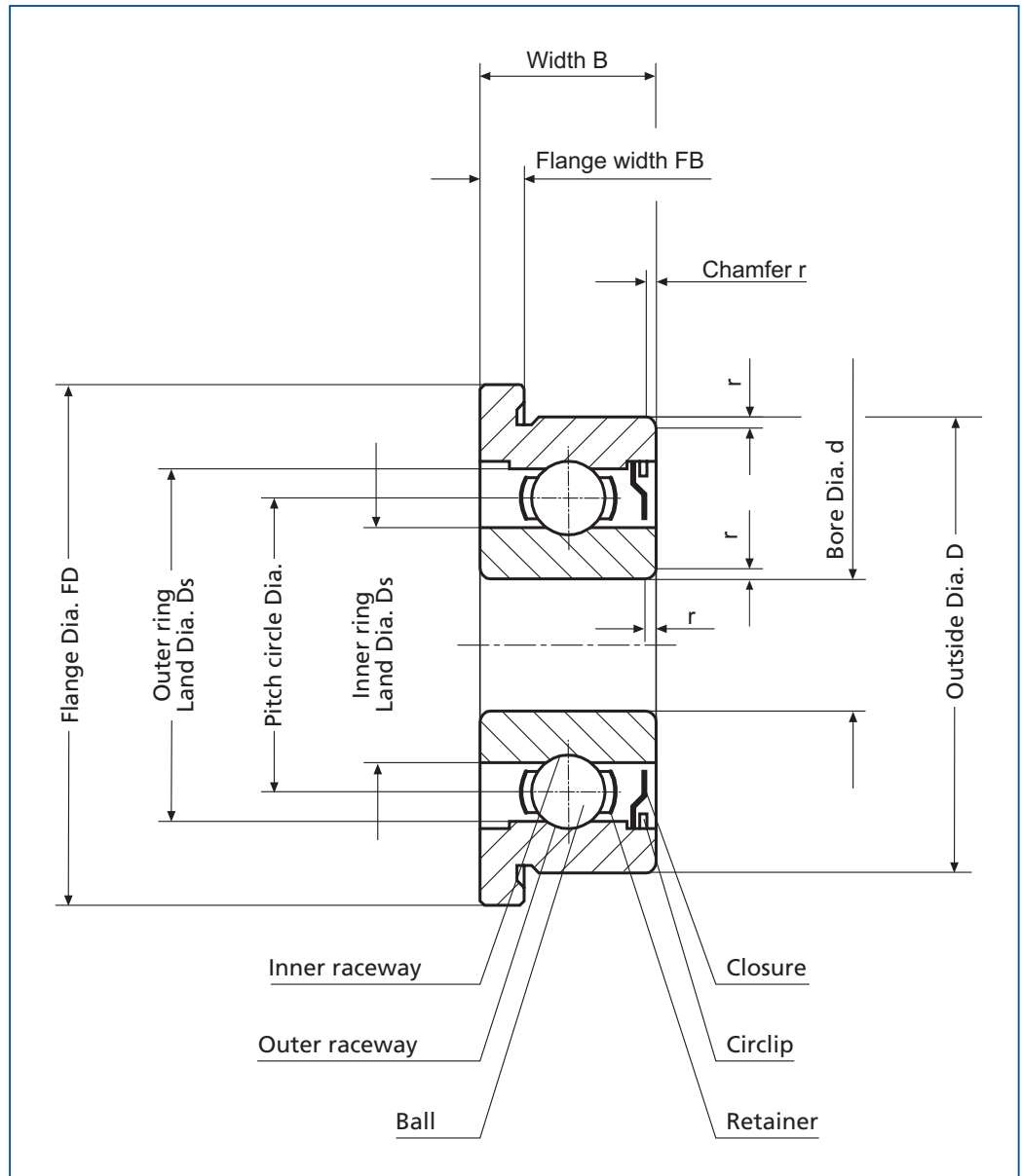
Fig. 28: Ball bearing parts
