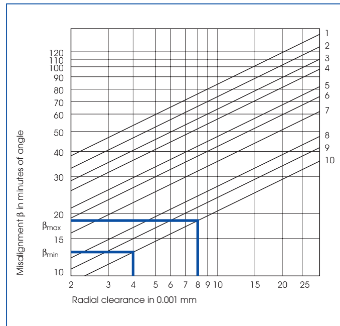
Figure 25: Misalignment calculation
