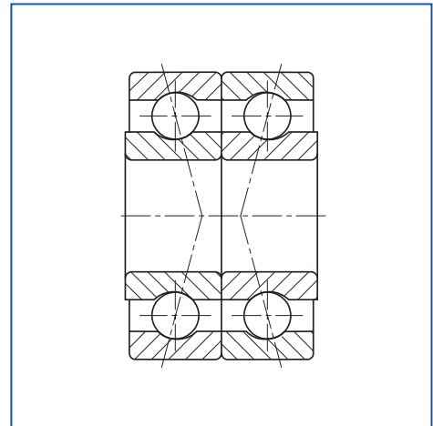
Figure 22: Face to face
